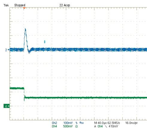
Step Load Transient Response (Vin=5V, Vout=1.8V, Cload=0, Iout=3A to 1.5A) Trace 2=Vout, 100 mV/div. Trace 4=Iout, 2.5A/div.
