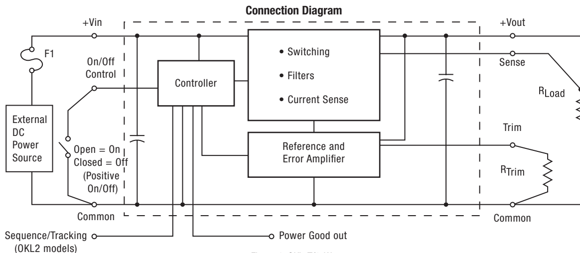
Figure 1. OKL-T/3-W5
