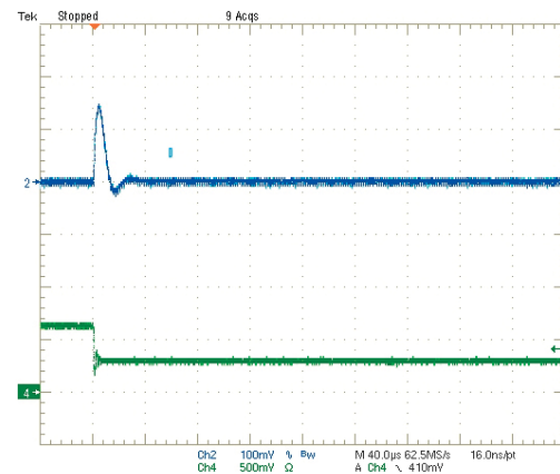
Step Load Transient Response (Vin=5V, Vout=0.6V, Load=0, Iout=3A to 1.5A) Trace 2=Vout, 100 mV/div. Trace 4=Iout, 2.5A/div.
