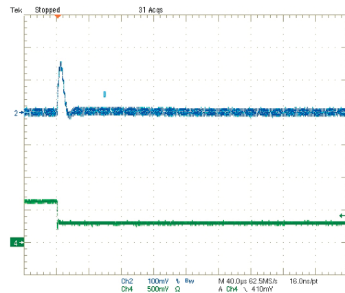
Step Load Transient Response (Vin=5V, Vout=2.5V, Load=0, Iout=3A to 1.5A) Trace 2=Vout, 100 mV/div. Trace 4=Iout, 2.5A/div.
