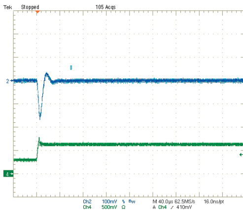
Step Load Transient Response (Vin=5V, Vout=0.6V, Load=0, Iout=1.5A to 3A) Trace 2=Vout, 100 mV/div. Trace 4=Iout, 2.5A/div.
