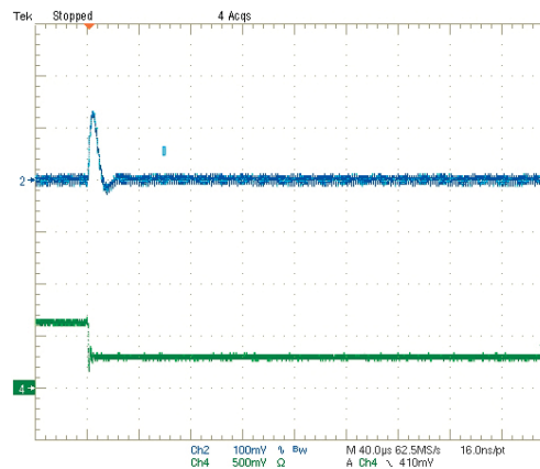
Step Load Transient Response (Vin=5V, Vout=1.2V, Clad=0, Iout=3A to 1.5A) Trace 2=Vout, 100 mV/div. Trace 4=Iout, 2.5A/div.
