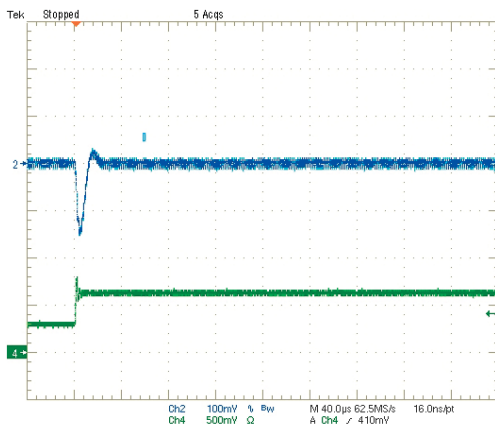
Step Load Transient Response (Vin=5V, Vout=1.5V, Clad=0, Iout=1.5A to 3A) Trace 2=Vout, 100 mV/div. Trace 4=Iout, 2.5A/div.
