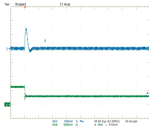
Step Load Transient Response (Vin=5V, Vout=1.5V, Clad=0, Iout=3A to 1.5A) Trace 2=Vout, 100 mV/div. Trace 4=Iout, 2.5A/div.
