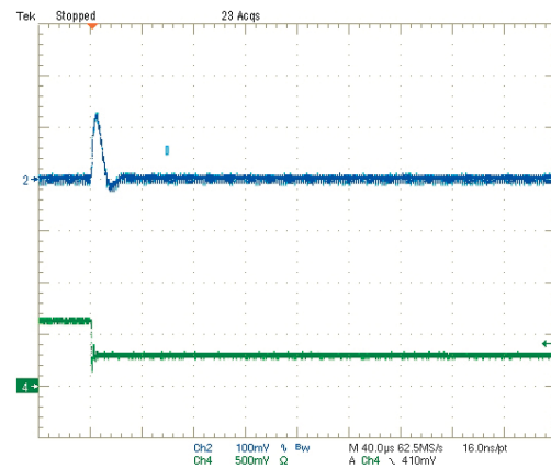
Step Load Transient Response (Vin=5V, Vout=1.0V, Load=0, Iout=3A to 1.5A) Trace 2=Vout, 100 mV/div. Trace 4=Iout, 2.5A/div.
