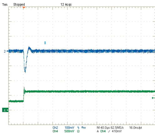
Step Load Transient Response (Vin=5V, Vout=1.2V, Clad=0, Iout=1.5A to 3A) Trace 2=Vout, 100 mV/div. Trace 4=Iout, 2.5A/div.
