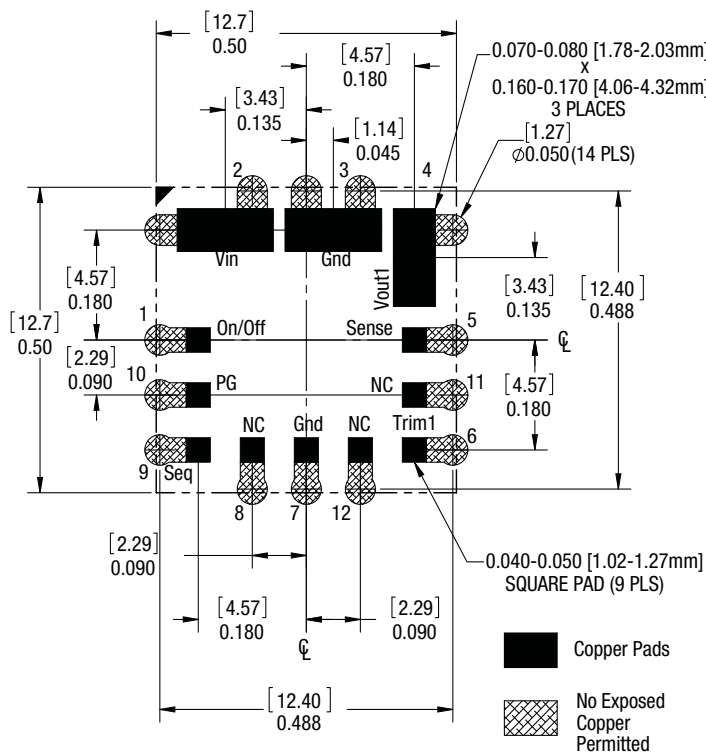
Figure 3. OKL-T/3-W5 Mechanical Outline
