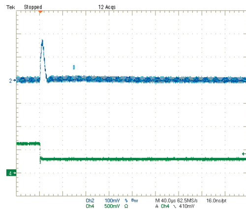
Step Load Transient Response (Vin=5V, Vout=3.3V, Load=0, Iout=3A to 1.5A) Trace 2=Vout, 100 mV/div. Trace 4=Iout, 2.5A/div.
