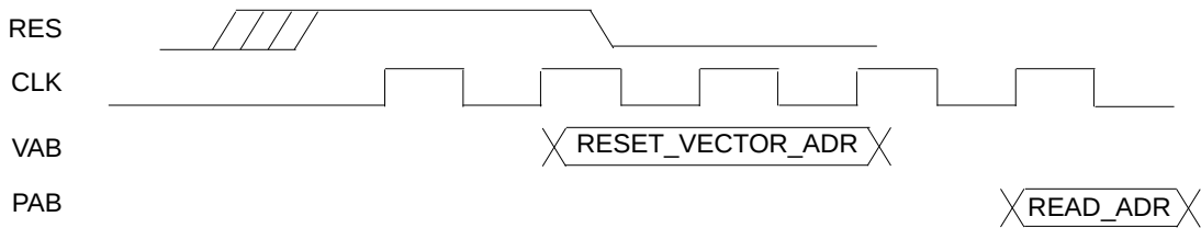
Figure 5-19 Reset Interface
