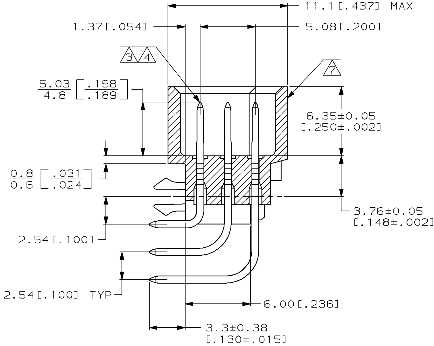
SECTION X-X
