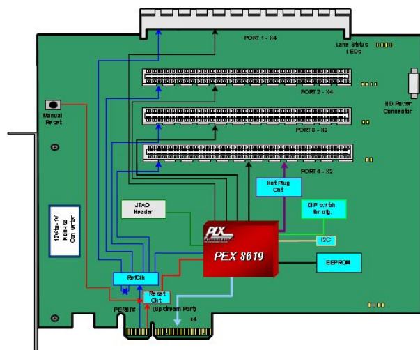
Figure 8. PEX 8619RDK
