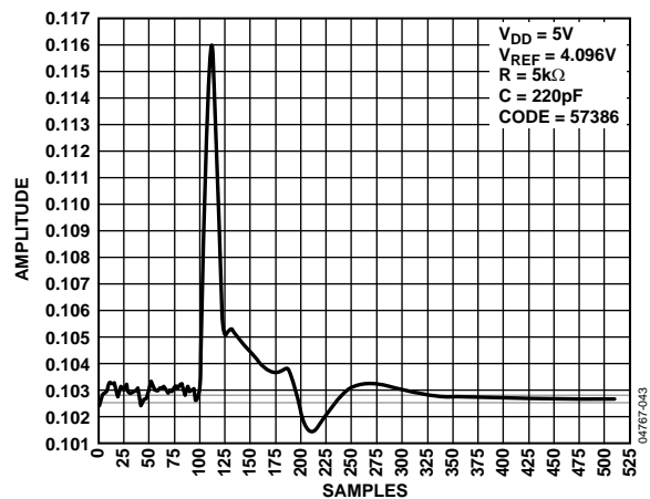
Figure 24. AD5060 Digital-to-Analog Glitch Energy
