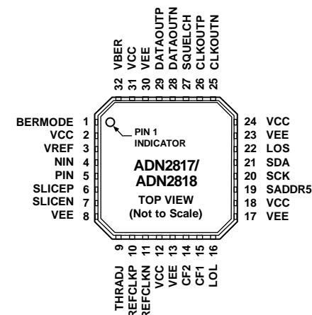
Figure 5. Pin Configuration
