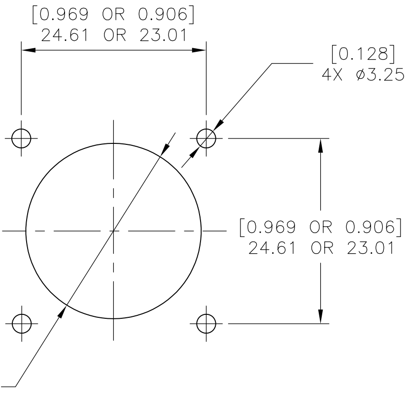
FRONT MOUNTING
