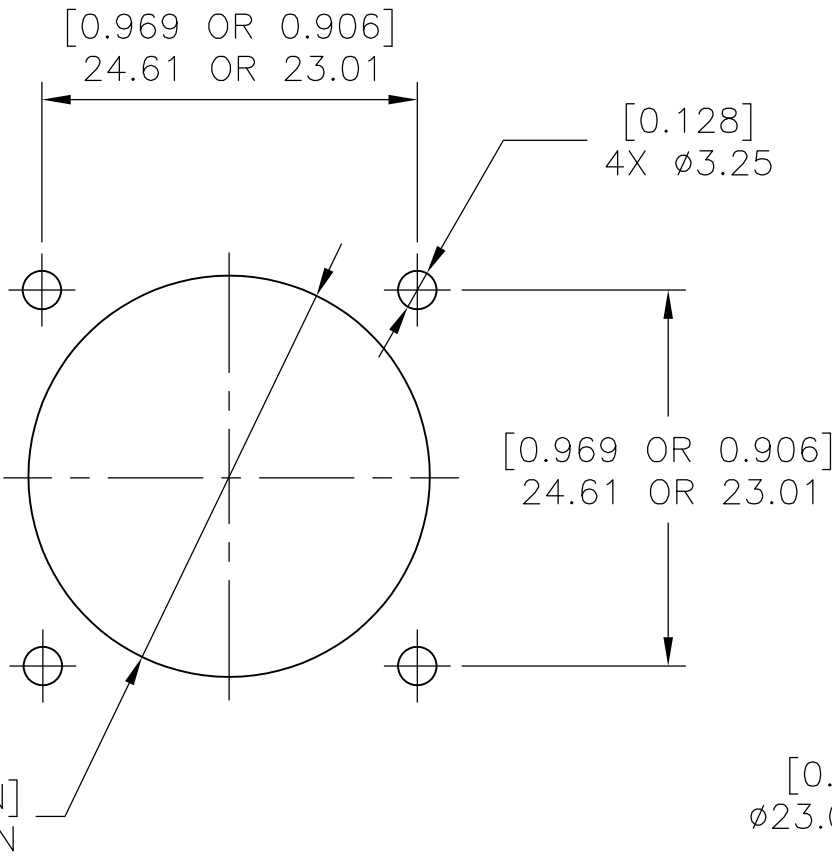
REAR MOUNTING
