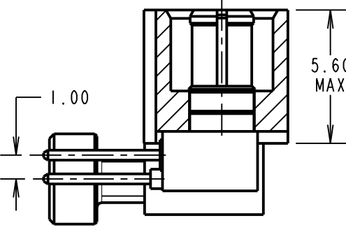
SECTION Z-Z
