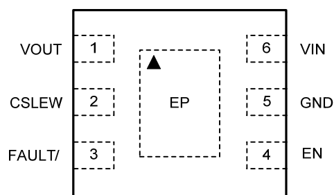
2mm x 2mm 6-pin Thin DFN (MT)
