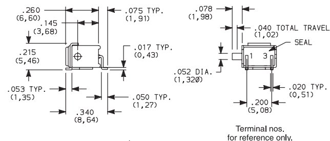
PC MOUNTING
