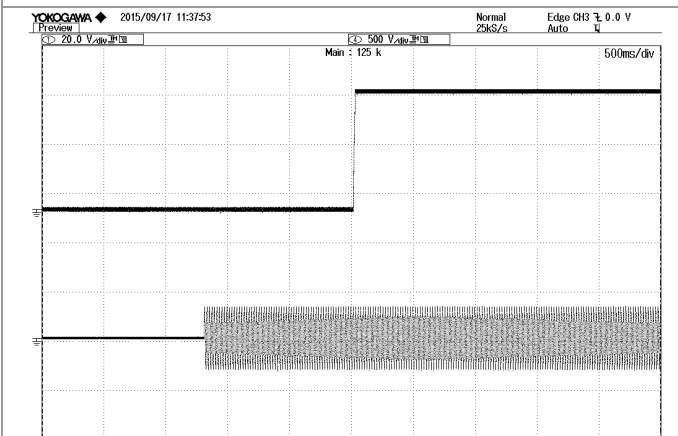
Figure 5: V_{out} start up with Enable on at 220Vac, 10.5A I_{out} , TOP: V_{out} , 20V/div, 500ms/div BOTTOM: V_{in} , 500V/div, 500ms/div
