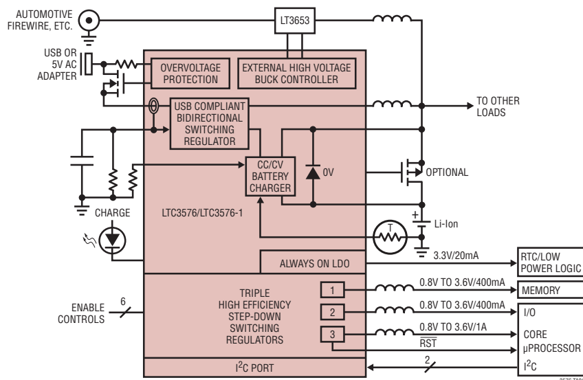
High Efficiency PowerPath Manager with Overvoltage Protection and Triple Step-Down Regulator
