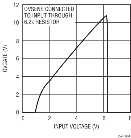
OVSTATE vs OVSENS
