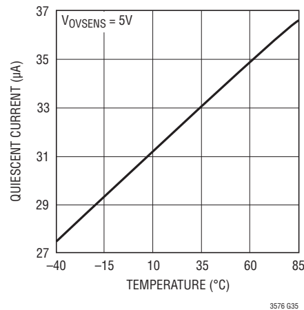
OVSTATE Quiescent Current vs Temperature
