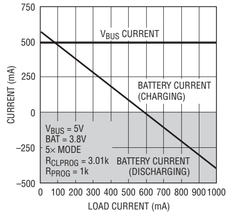
Battery and V_{BUS} Currents vs Load Current
