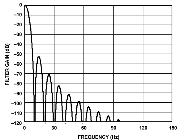
Figure 34. \text{Sinc}^4 Filter Response (FS[9:0] = 480)
