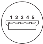
Pin assignment plug USB, type A
