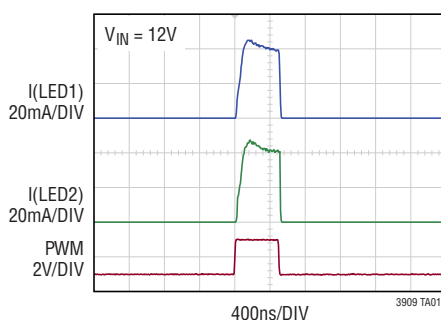
LED Current Waveforms 20,000:1 PWM Dimming (100Hz)
