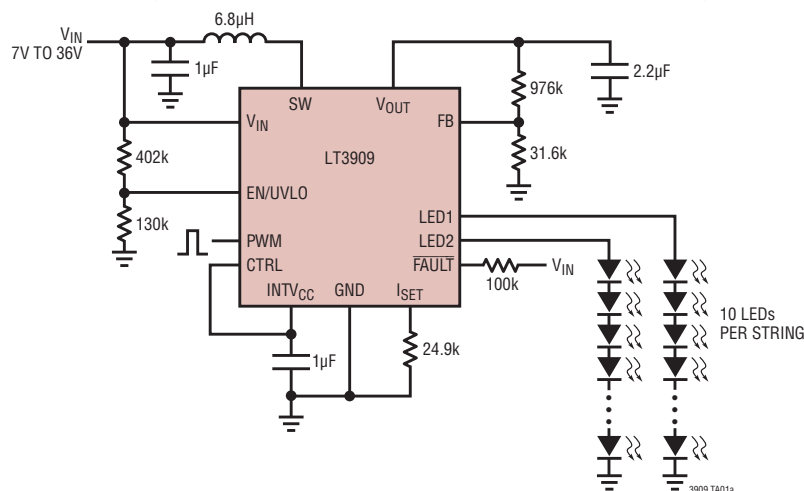
2-String x 40mA, 2MHz LED Driver for Ten White LEDs/String
