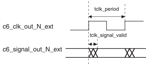
Figure 12. CSIX Outbound AC Timing Specifications
