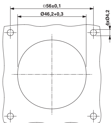
Dimensional drawing
