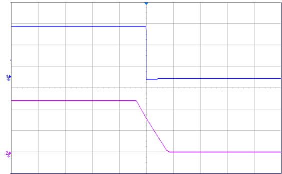
Figure 7 Output voltage shutdown by power-off, (100ms/div), see Figure 11 for test configuration; CH1-output voltage (500mV/div); CH2-input voltage (20V/div)
