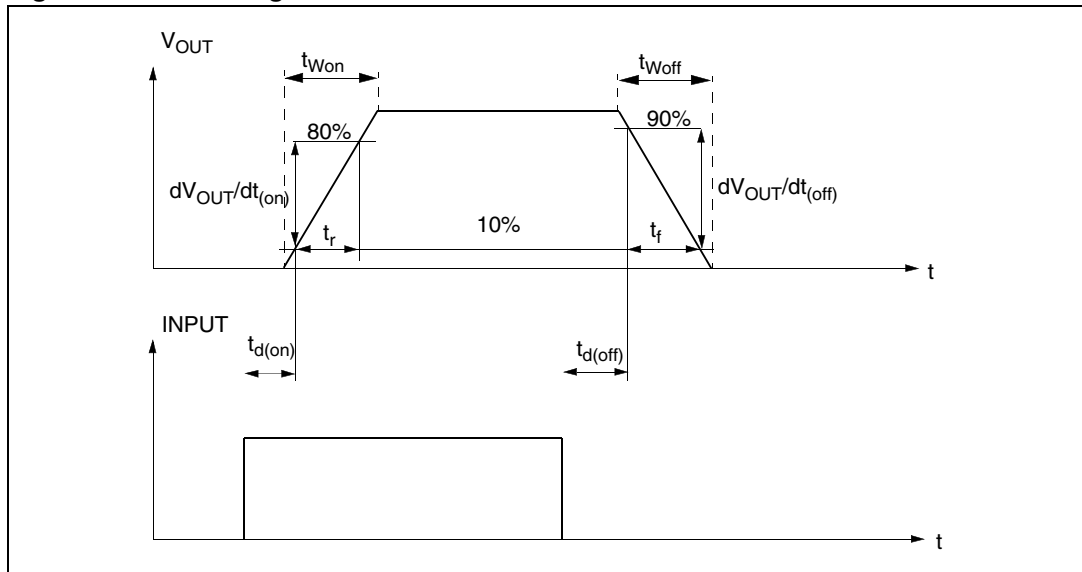
Figure 5. Switching characteristics
