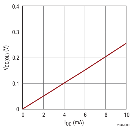
GPIO, SDAO, SDAO Loaded Output Low Voltage vs Load Current
