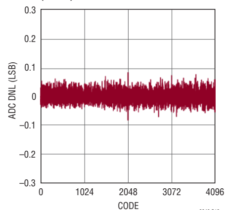
ADC Differential Nonlinearity (ADIN)
