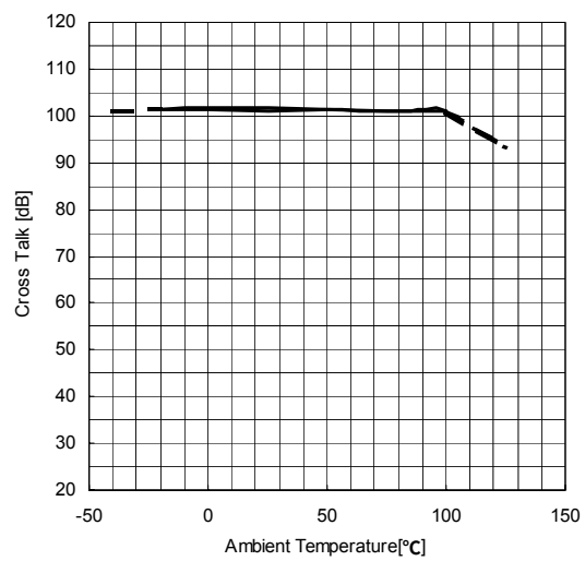
Cross Talk vs. Ambient Temperature Input : L1, Output : FL, Rg=0Ω, BW:400Hz-30kHz
