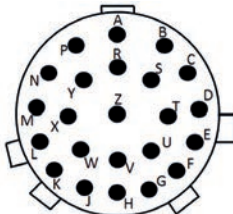
Shell Size 18 23
