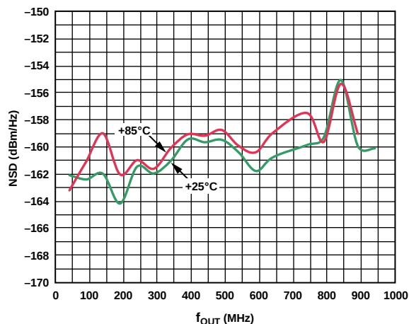
Figure 29. Single-Tone NSD vs. f_{OUT} over Temperature
