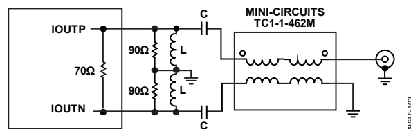
Figure 184. Recommended Mix-Mode Configuration Offering Extended RF Bandwidth Using a TC1-1-462M Balun
