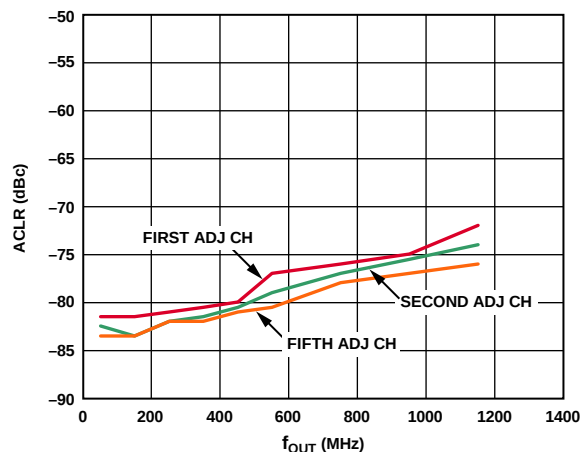
Figure 32. Single-Carrier WCDMA ACLR vs. f_{OUT} at 2457.6 MSPS
