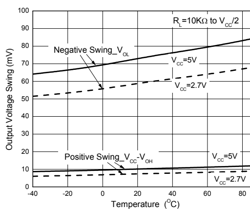
Figure 16. Output Voltage Swing vs. Temperature
