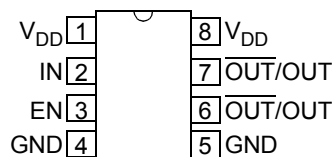
MCP14A1201/MCP14A1202 MSOP/SOIC
