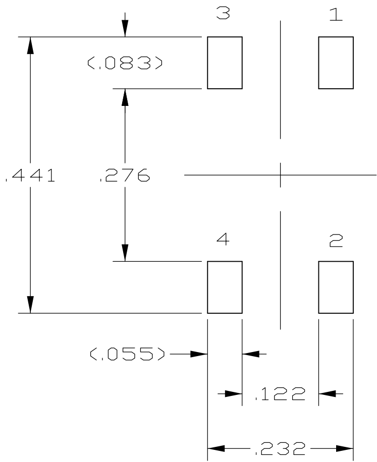
RECOMMENDED PAD LAYOUT TOLERANCE ±.002 UNLESS OTHERWISE NOTED
