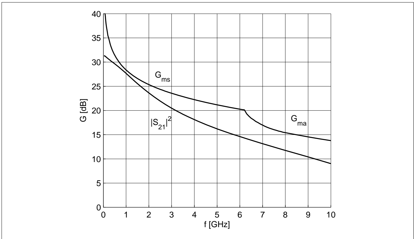
Figure 5-12 Gain G_{ma}, G_{ms}, |S_{21}|^2 = f(f), V_{CE} = 3 \text{ V}, I_C = 15 \text{ mA}
