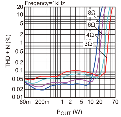
THD+N vs. Pout
