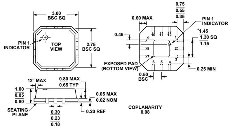
Figure 28. 12-Lead Lead Frame Chip Scale Package (LFCSP_VQ) 3 mm × 3 mm Body, Very Thin Quad (CP-12-1)
