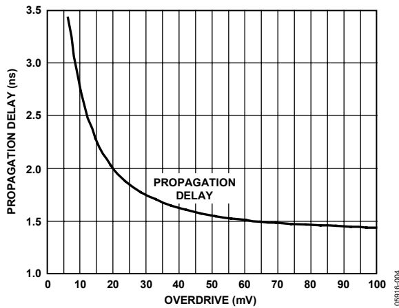
Figure 12. Propagation Delay vs. Input Overdrive
