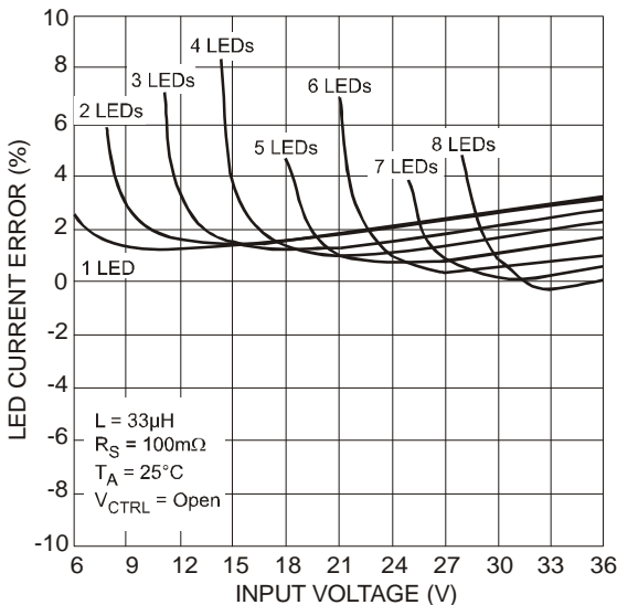
Figure 29 LED Current Deviation vs. Input Voltage
