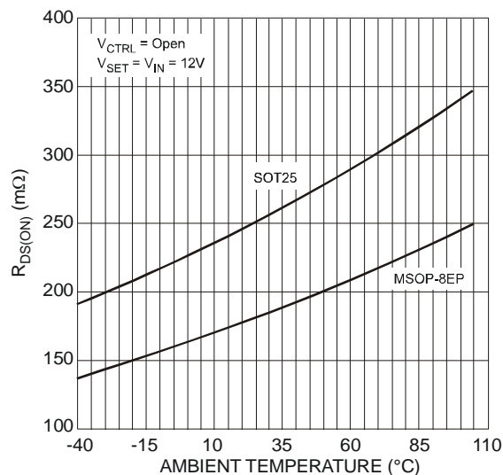
Figure 6 SW R_{DS(ON)} vs. Temperature
