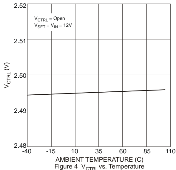
Figure 4 V_{CTRL} vs. Temperature
