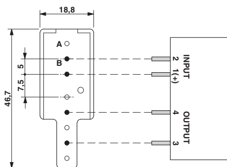
Dimensioned drawing
