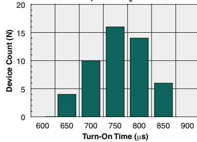
Typical Turn-On Time Distribution (N=50, I F =5mA, I L =60mA)
