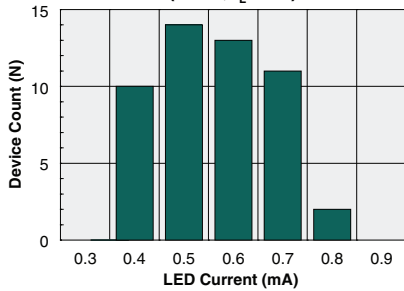
Typical I F for Switch Operation (N=50, I L =120)
