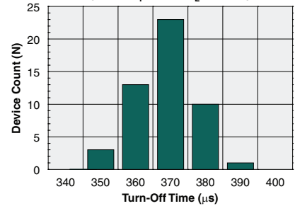
Typical Turn-Off Time Distribution (N=50, I F =5mA, I L =60mA)
