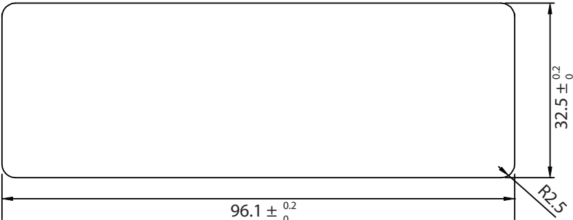
PANEL CUTOUT
