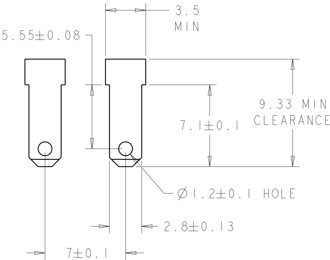
SCALE 5:1 MATING TAB DIMENSIONS
