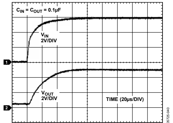
Figure 36. ADR125 Turn-On Response
