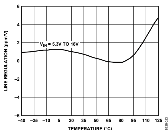
Figure 19. ADR125 Line Regulation vs. Temperature
