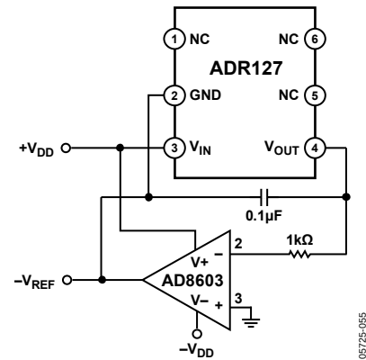
Figure 51. Negative Reference
