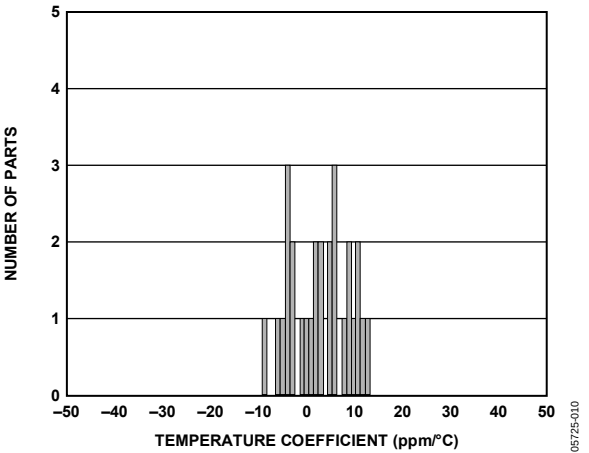
Figure 6. ADR125 Temperature Coefficient
