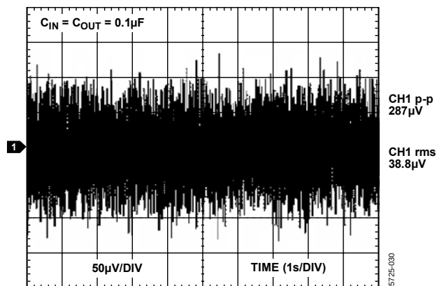
Figure 26. ADR127 10 Hz to 10 KHz Noise
