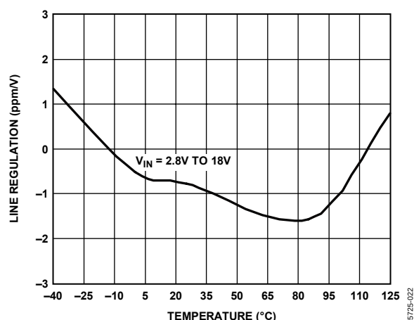
Figure 18. ADR121 Line Regulation vs. Temperature
