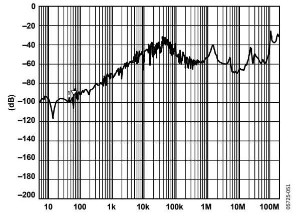
Figure 47. ADR121/ADR125/ADR127 PSRR
