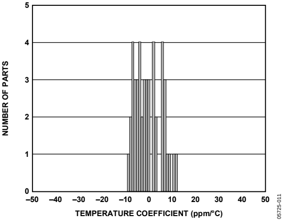
Figure 7. ADR121 Temperature Coefficient
