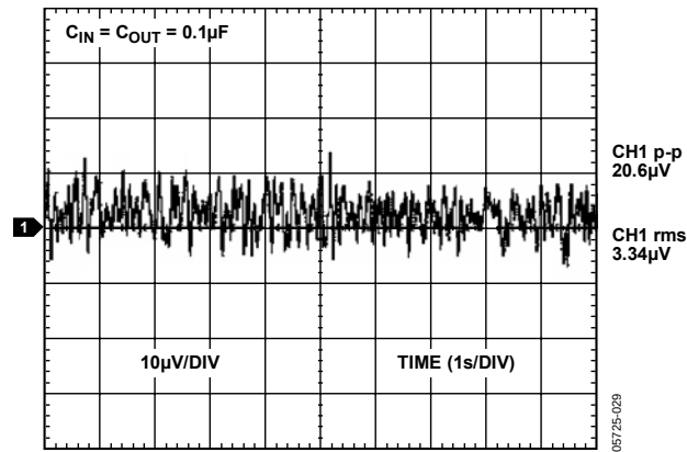
Figure 25. ADR125 0.1 Hz to 10 Hz Noise
