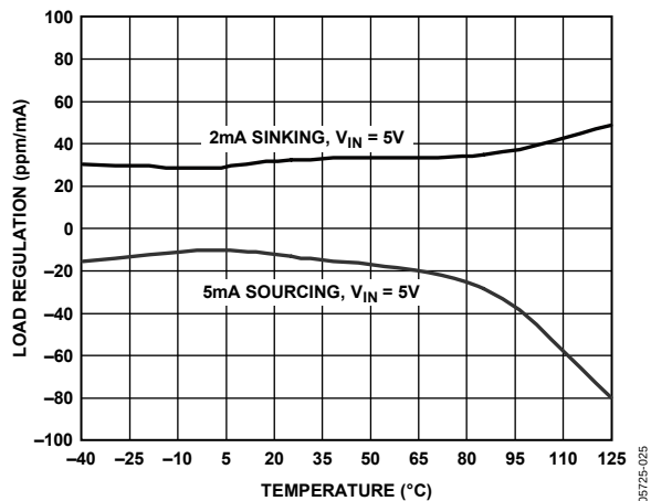
Figure 21. ADR121 Load Regulation vs. Temperature
