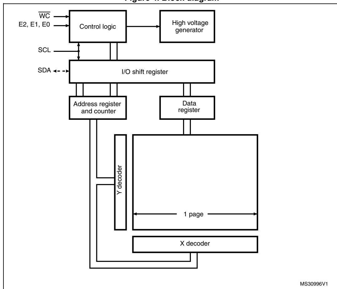
Figure 4. Block diagram
