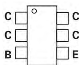
Pin-Out Top
