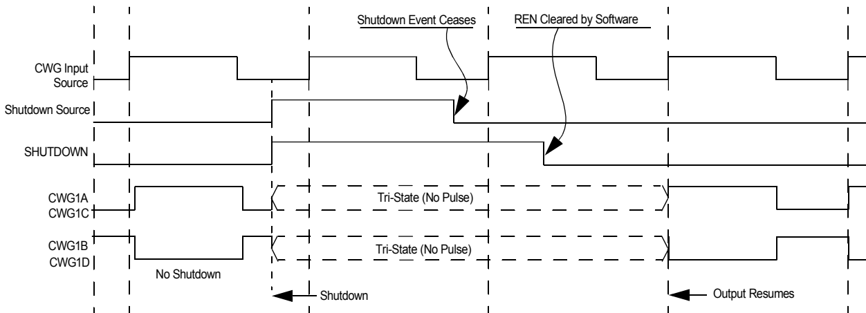
Figure 24-17. SHUTDOWN FUNCTIONALITY, AUTO-RESTART DISABLED (REN = 0, LSAC = 01, LSBD = 01)
