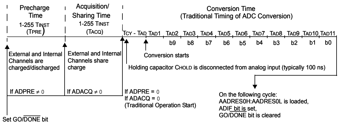
Figure 31-10. Hardware CVD Sequence Timing Diagram
