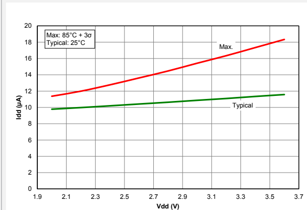
Figure 39-65. I_{PD} , Brown-out Reset, BORV = 1, PIC18LF24/25K40 only
