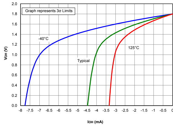
Figure 39-98. V_{OH} vs I_{OH} , Over Temperature, V_{DD} = 5.0V , PIC18LF24/25K40 only
