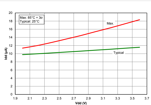
Figure 39-65. I_{DD} , Brown-out Reset, BORV = 1, PIC18LF24/25K40 only
