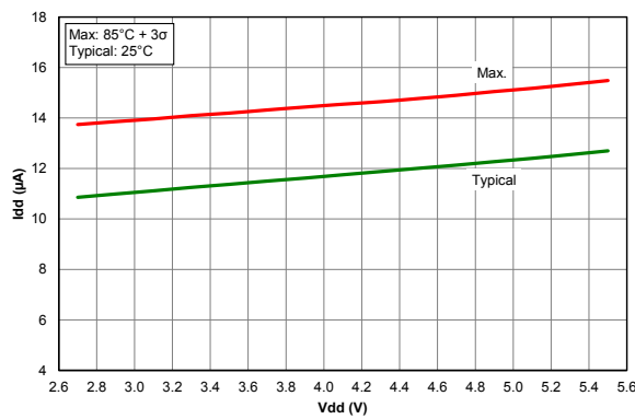
Figure 39-68. I_{PD} , Low-power Brown-out Reset, LPBOR = 0, PIC18F24/25K40 only
