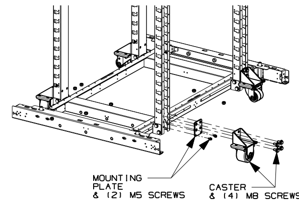
TYPICAL CASTER MOUNTING - 4 PLCS
