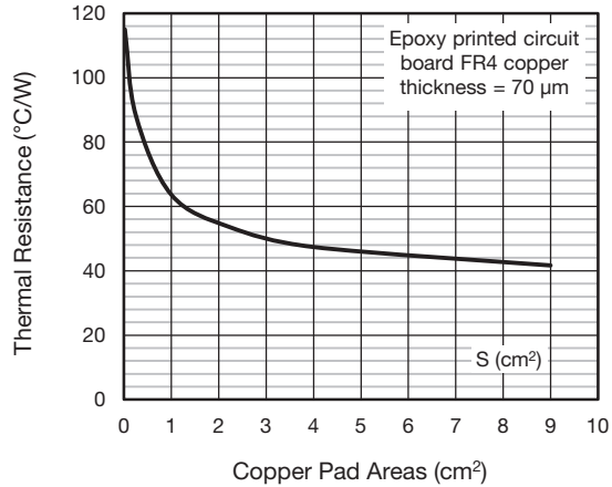
Fig. 7 - Thermal Resistance Junction to Ambient vs. Copper Pad Area
