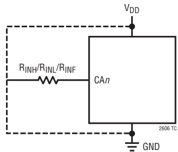
Test Circuit 2
