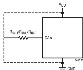
Test Circuit 2
